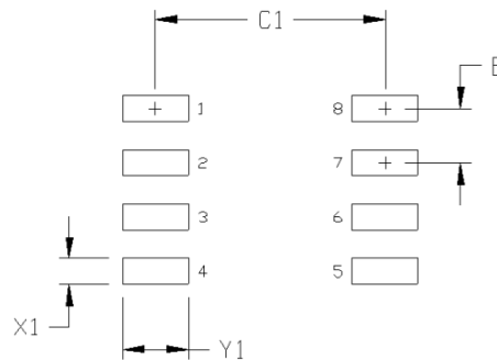
Figure 19. 8-Lead Narrow Body SOIC [NB SOIC-8] Land Pattern
