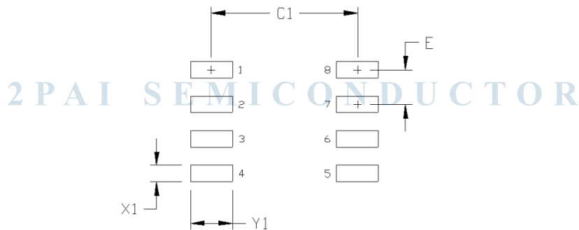
Figure 24. 8-Lead Narrow Body SOIC [NB SOIC-8] Land Pattern
