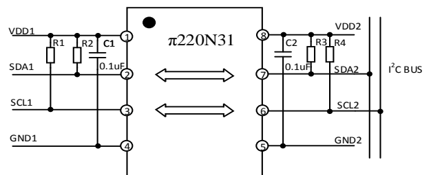
Figure2. \pi 220N31 Typical Application Circuit
